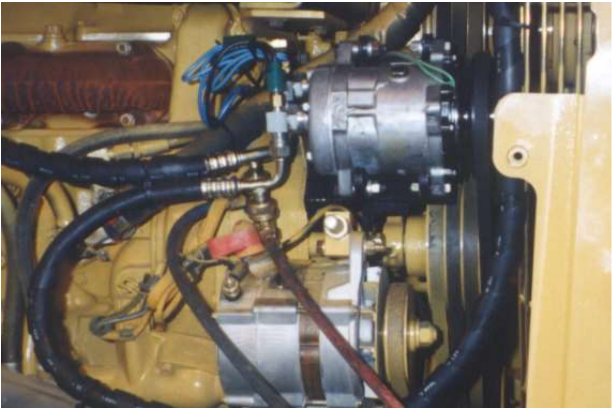
Compressor mount and compressor in place.
