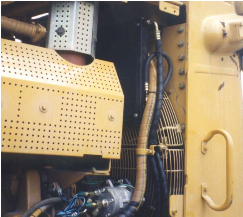
Hoses into evaporator box with clutch wire in background.
