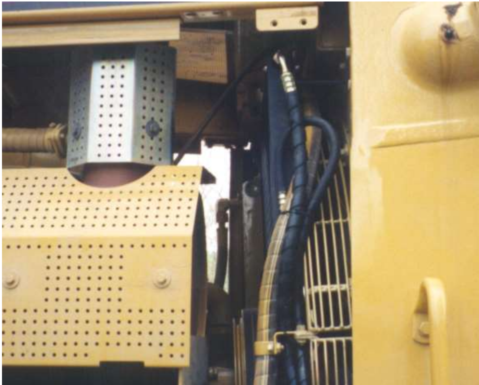
Right side of condenser in place with hoses and fittings.
